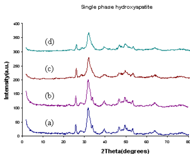
Fig.2. XRD patterns of synthesized HAp, a. in the absence of polymer, b. in the presence of 0.2g starch, c. in the presence of 0.5g starch, and d. in the presence of 0.8g starch
