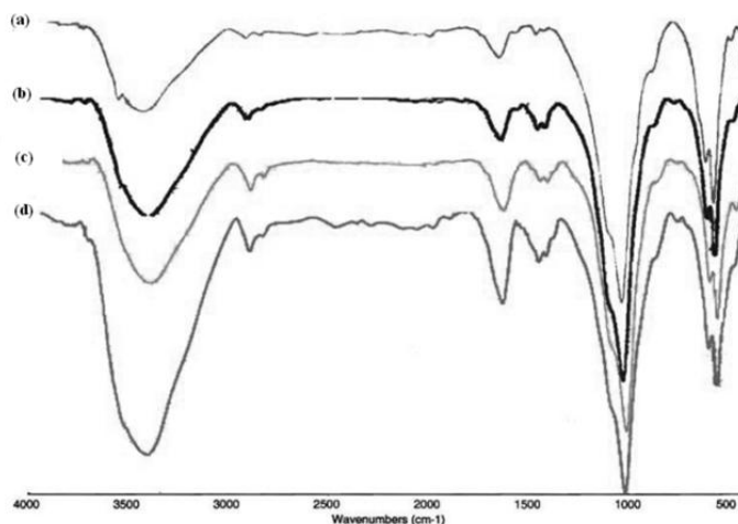
Fig.1. IR spectra of synthesized HAp , a. in the absence of polymer, b. in the presence of 0.2g starch, c. in the presence of 0.5g starch, and d. in the presence of 0.8g starch
