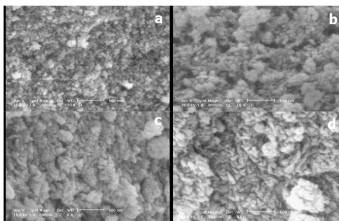
Fig.3. SEM micrographs of synthesized HAp, a. in the absence of polymer, b. in the presence of 0.2g starch, c. in the presence of 0.5g starch, and d. in the presence of 0.8g starch
