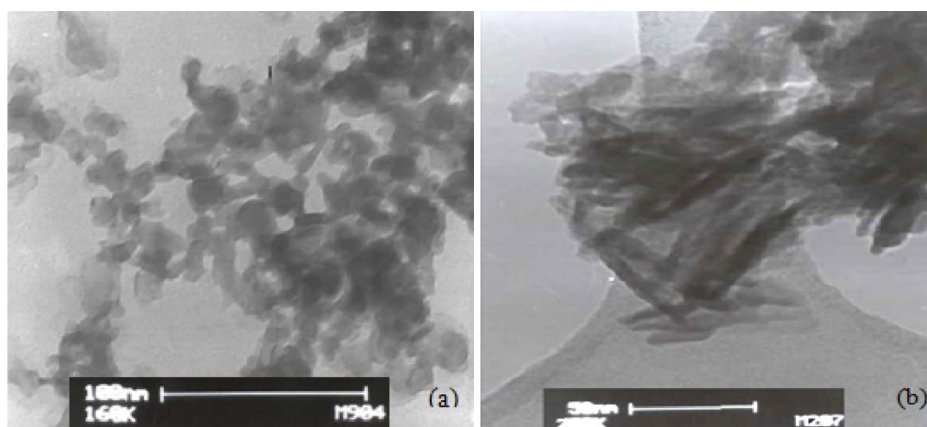
Fig.4. TEM micrographs of synthesized HAp, a. in the absence of polymer, and b. in the presence of 0.8 g starch
