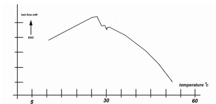
Fig.11. DSC spectra of the grafted polystyrene by gamma ray (radiation dose: 40 KGy)
