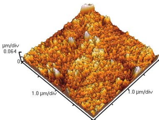
Fig.10. Atomic force microscopy of grafted polystyrene under 30 KGy. (scale: 1 \times 1 \mu\text{m} )
