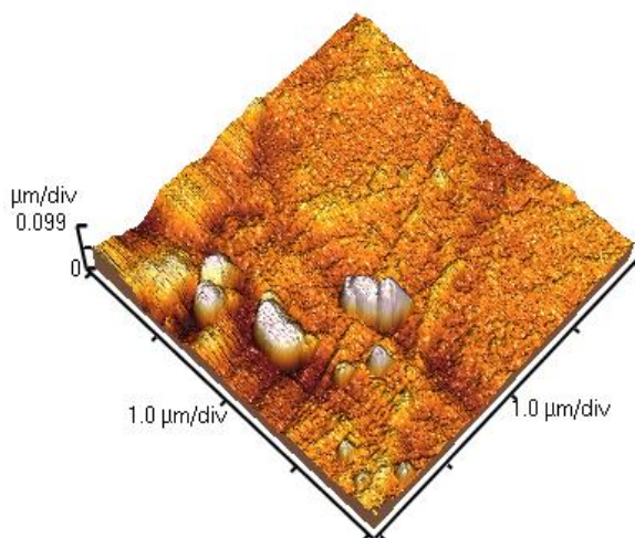
Fig.4. Atomic force microscopy of grafted polystyrene under 10 KGy. (scale: 1 \times 1 \mu\text{m} )
