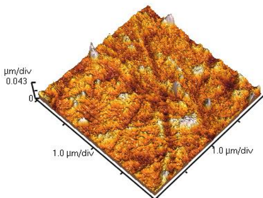
Fig.6. Atomic force microscopy of grafted polystyrene under 20 KGy. (scale: 1 \times 1 \mu\text{m} )
