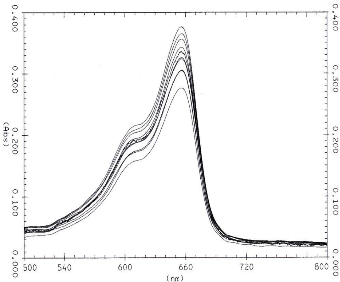
Fig.2. UV-visible spectra of the reduction of MB by varying amounts of ammonia in TX-100 micelle.
