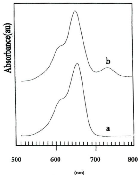
Fig. 3. Electronic spectra of MB in : (a) water and (b) hydrochloric acid
