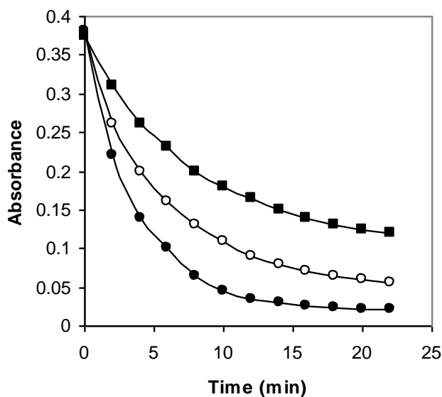
Fig.4. Absorbance vs. time plot for the reduction of MB by ammonia in (a) TX-100, (b) Na-MOR and (c) Nanomordenite.
