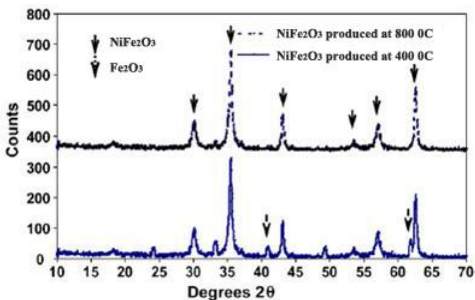
Fig.3. XRD diagram to check the size of nanoparticles synthesized nanoparticle synthesis
