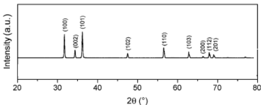
Fig.4. XRD patterns of Zn_{0.97}Co_{0.03}O photocatalysts
