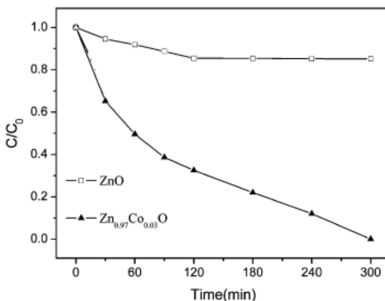
Fig.5. Photocatalytic decolorization kinetics of MB using Zn_{0.97}Co_{0.03}O photocatalysts
