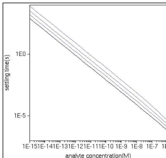
Fig.8. Settling time vs. analyte concentration for a nanosphere sensor
