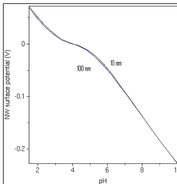
Fig.4. Conductance modulation vs. pH of a nanowire sensor
