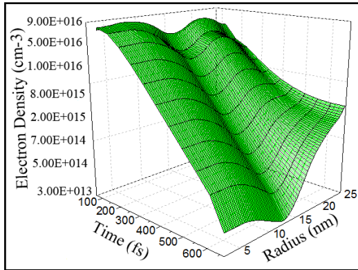
Fig. 6. 3D surface of time evolution of the electron density for active region in logarithmic scale
