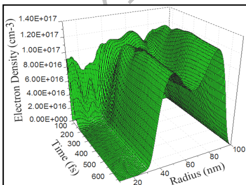
Fig. 5. 3D surface of time evolution of the electron density in a closed system
