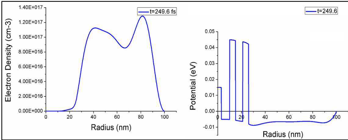
D3. Time evolution of the electron density in t=249.6 fs
