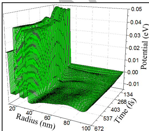
Fig. 7. 3D surface of time evolution of the potential in a closed system
