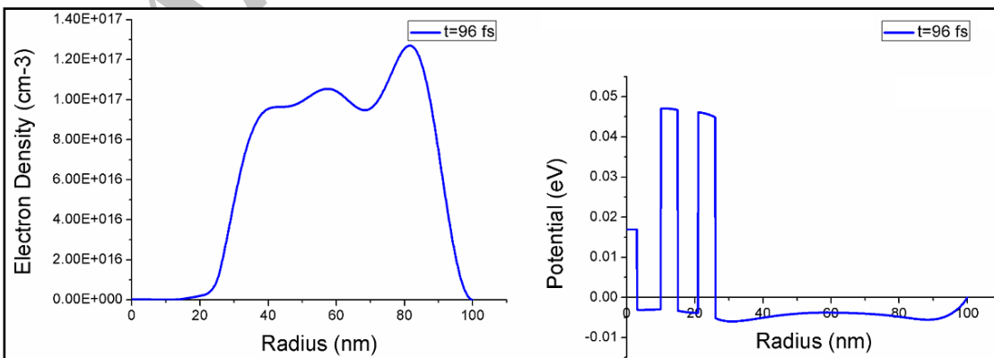
C3. Time evolution of the electron density in t=96 fs
