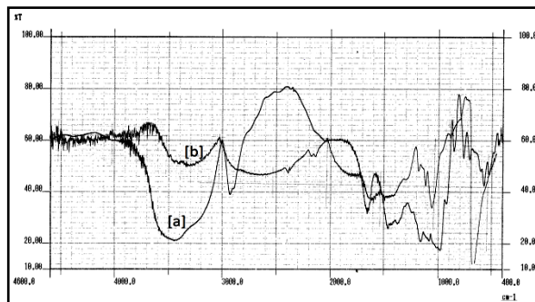
Fig. 4. (a): IR Spectra of pure starch. (b): IR Spectra of CuO nanoparticle
