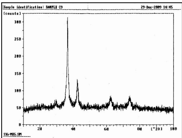
Fig. 1. XRD spectra of Prepared CuO nanoparticle.
