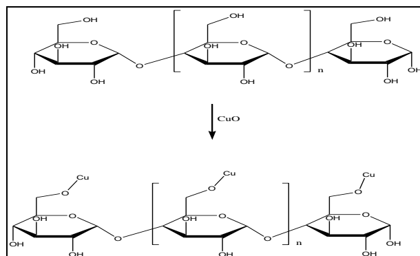
Fig. 5. Possible chemical bonding between CuO and Starch.
