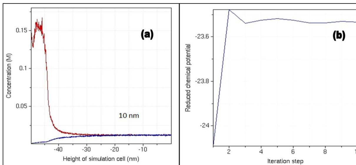
Fig. 2. (a) Na + and Cl - concentration with height of the simulation cell and (b) reduced chemical potential with the iteration step when the simulation cell contains 4 dsDNA oligomers with voltage= -50 mV, distance between the molecules=8nm and the length of the molecules is 16 bases.
