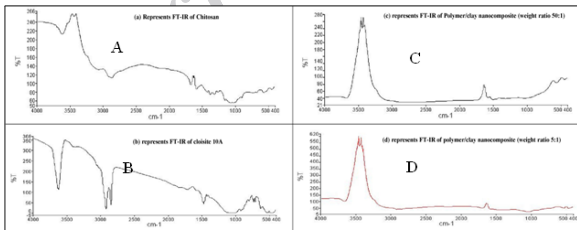
Fig. 1. FT-IR spectra of cloisite(A), cloisite 10A(B), Polymer/clay nanocomposite (weight ratio 50:1) (C) and polymer/clay nanocomposite (weight ratio 5:1) (D).
