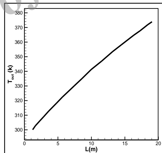
Fig. 7. Mean outlet temperature variation with receiver length.
