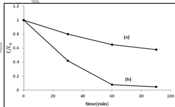
Fig. 6. Photocatalytic degradation using pure (a) TiO 2 and (b) La,S-TiO 2 .
