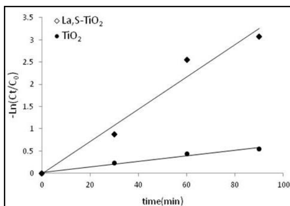
Fig. 7. Kinetic analysis with \text{La,S-TiO}_2 and \text{TiO}_2
