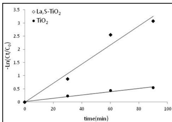
Fig. 7. Kinetic analysis with \text{La,S-TiO}_2 and \text{TiO}_2
