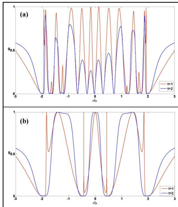
Fig. 3. Dimensionless conductance versus Fermi energy a) P=8 , R=9 and b) R=P=4 , with V_c = \mu , \varepsilon_0=0 & \varphi=0.3
