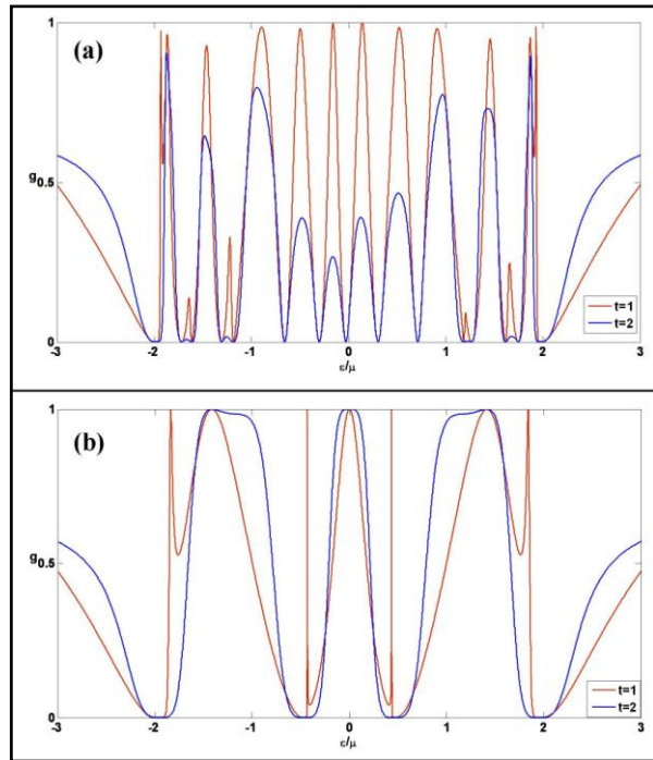
Fig. 3. Dimensionless conductance versus Fermi energy a) P=8, R=9 and b) R=P=4, with V_c = \mu , \epsilon_0=0 & \varphi=0.3
