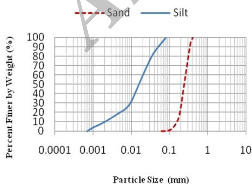
Fig. 1: Grain size distribution for Firoozkooch No.161 sand and Firoozkooch silt.
