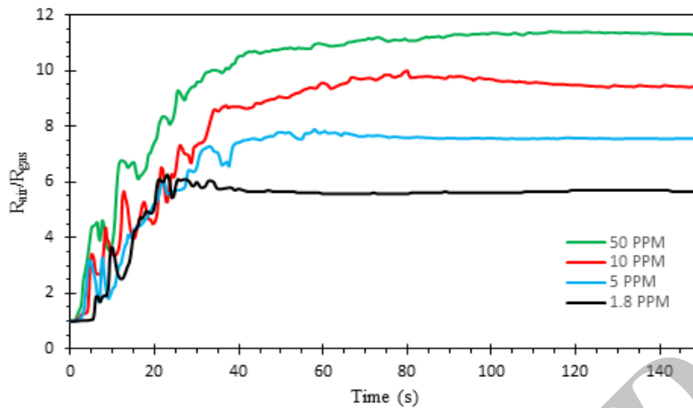
Fig. 12: Gas response of the WO 3 microsphere based sensor to different concentrations of acetone at 300 °C.
