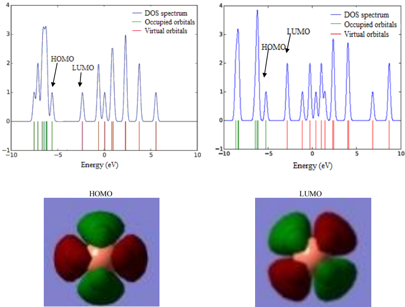
Fig. 3: DOS of \text{Cu}_2 nanocluster (Left), DOS, HOMO and LUMO pictures of \text{Cu}_2\text{CO} complex (Right).
