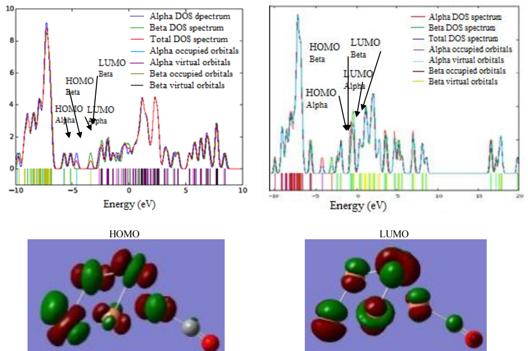
Fig. 8: DOS of \text{Cu}_7 nanocluster (Left), DOS, HOMO and LUMO pictures of \text{Cu}_7\text{CO} complex (Right).
