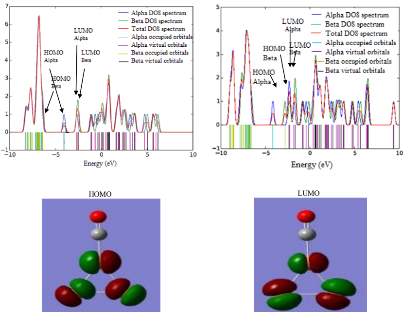
Fig. 4: DOS of \text{Cu}_3 nanocluster (Left), DOS, HOMO and LUMO pictures of \text{Cu}_3\text{CO} complex (Right).
