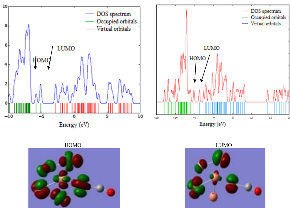
Fig. 9: DOS of Cu 8 nanocluster (Left), DOS, HOMO and LUMO pictures of Cu 8 CO complex (Right).
