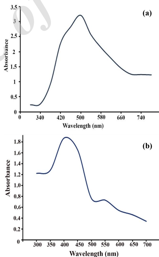
Fig. 2: UV-Vis spectra of silver nanoparticles synthesized by selected taxa of Cynanchum . a) spectrum of C. viminalis ; b) spectrum of C. sarcomedium .
