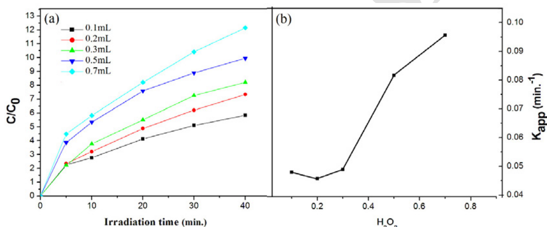
Fig. 10. (a) The effect of H_2O_2 on photodegradation of Malachite Green. (b) Kinetics data of photocatalytic degradation. Dye concentration = 10 mg L -1 , T=298K, initial amount of catalyst=0.01g.
