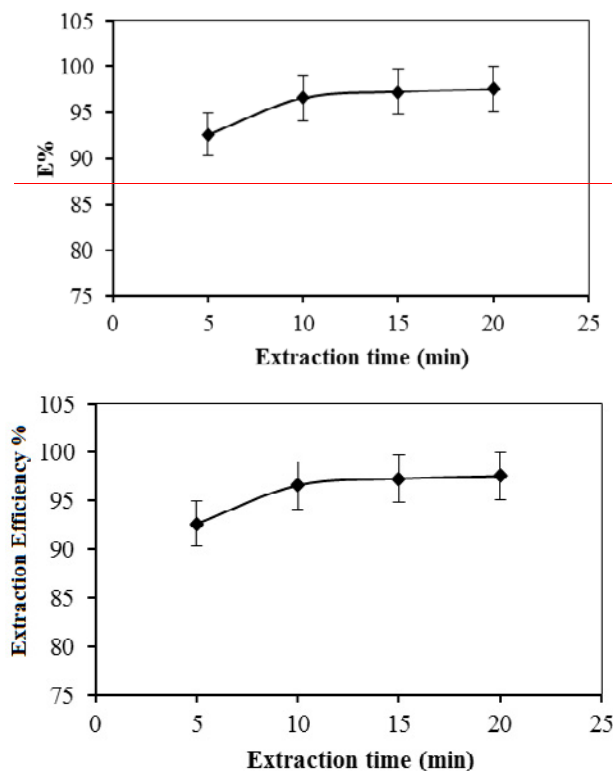
Fig. 5. Effect of extraction time on the percent of extraction of \text{Cu}^{2+} ions.
