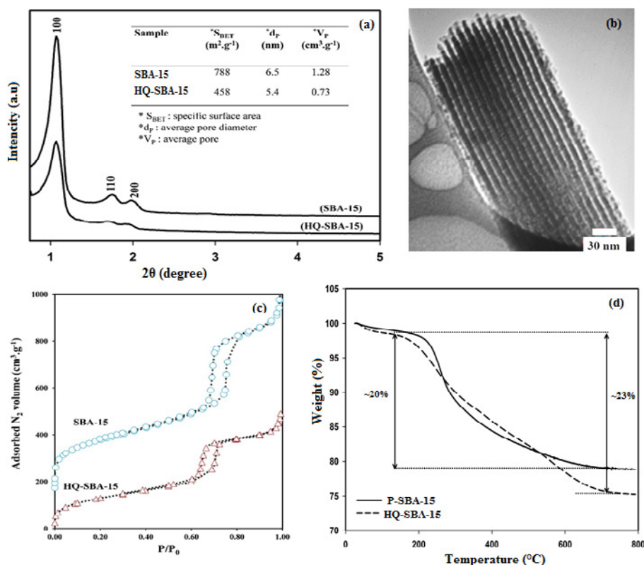
Fig. 2. a. XRD diffractions and textural parameters of SBA-15 and HQ-SBA-15, b. TEM images of SBA-15, c. \text{N}_2 adsorption-desorption isotherms of SBA-15 and HQ-SBA-15, and d. TGA curves of P-SBA-15 and HQ-SBA-15.
