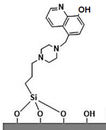
Fig. 1. Structure of 8-hydroxyquinoline grafted on SBA-15 (HQ-SBA-15).
