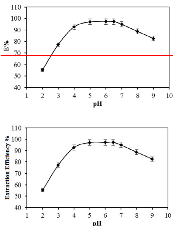
Fig. 3. Effect of pH on the percent of extraction of Cu 2+ ions.
