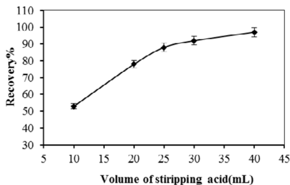
Fig. 6. Effect of volume of stripping acid on the percent of recovery of Cu 2+ ions.
