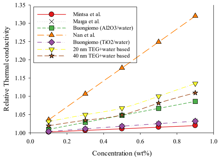
Fig. 13. Experimental data at 60 °C compared to empirical correlations at various concentrations.
