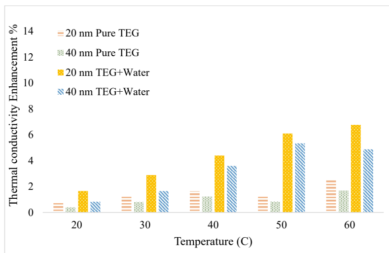
Fig. 11. Thermal conductivity enhancement of 0.5 wt.% samples at various temperatures.
