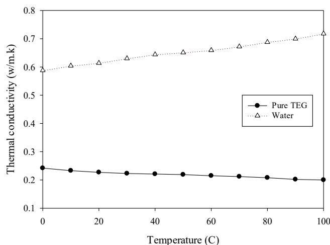
Fig. 6. Thermal conductivity for pure water and pure TEG at various temperatures [43].
