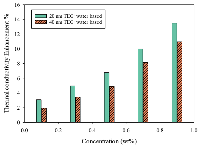
Fig. 8. Thermal conductivity enhancement for various nanofluid concentrations at 60 °C.
