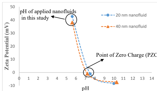
Fig. 3. Effects of pH on the zeta potential of TEG-water based nanofluids.
