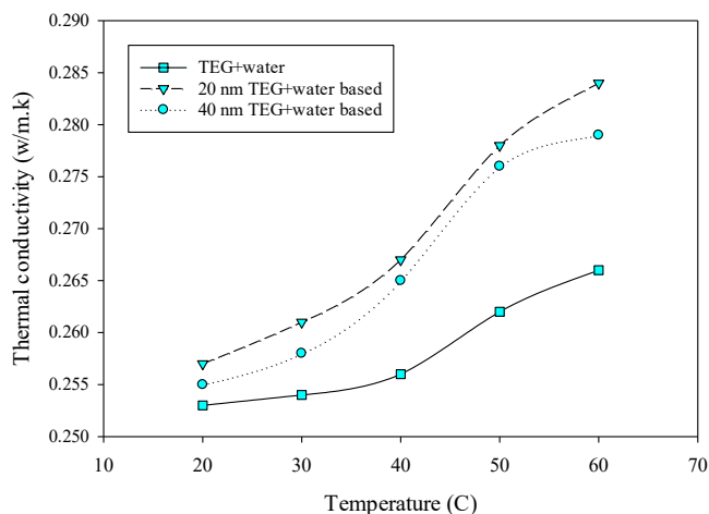
Fig. 5. Thermal conductivity for 0.5 wt.% nanofluids at various temperatures.
