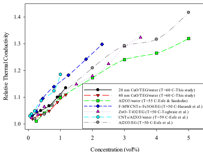
Fig. 14. Experimental data at 60 °C compared to other experimental studies in the literature using KD 2 pro thermal analyzer at various concentrations [57-61].
