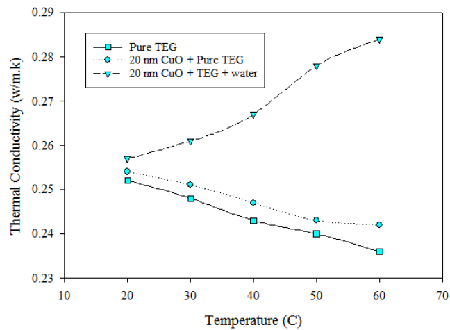
Fig. 9. Thermal conductivity of pure TEG and 20 nm, 0.5 wt.% samples at various temperatures.
