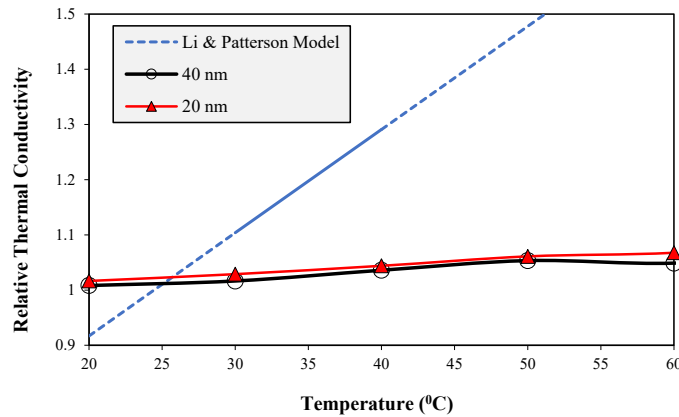
Fig. 12. Relative thermal conductivity for 0.5 wt.% nanofluids compared with Li & Peterson model.
