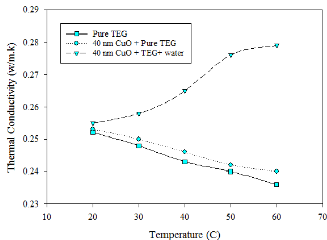
Fig. 10. Thermal conductivity of pure TEG and 40 nm, 0.5 wt.% samples at various temperatures.
