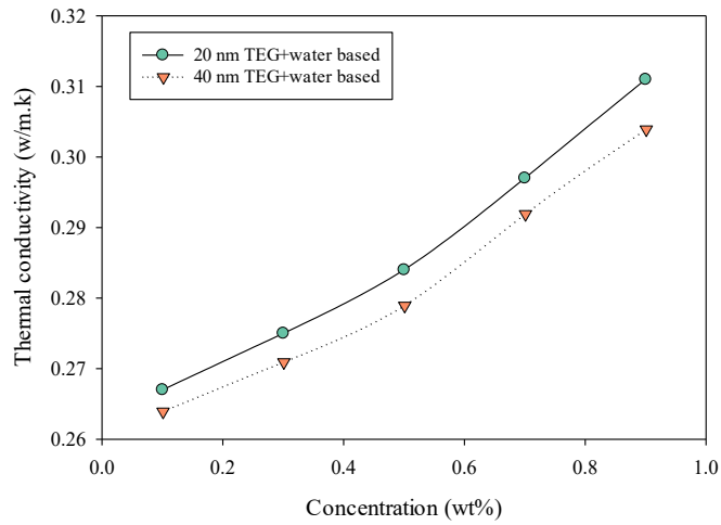
Fig. 7. Thermal conductivity value for various nanofluid concentrations at 60 °C.
