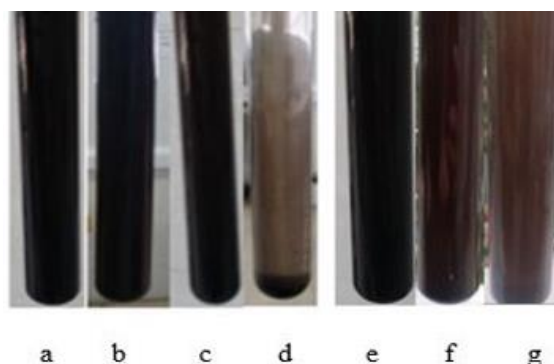
Fig. 2. TEG-water based nanofluid contained TX-100 at the first day (a), TX-100 is still stable on the next day (b), TX-100 is still stable during a 10-day period (c) and TX-100 within two weeks (d). Pure TEG based nanofluid contained TEAOH on the first day (e), on the next day (f) and is still stable during a 3-day period (g).
