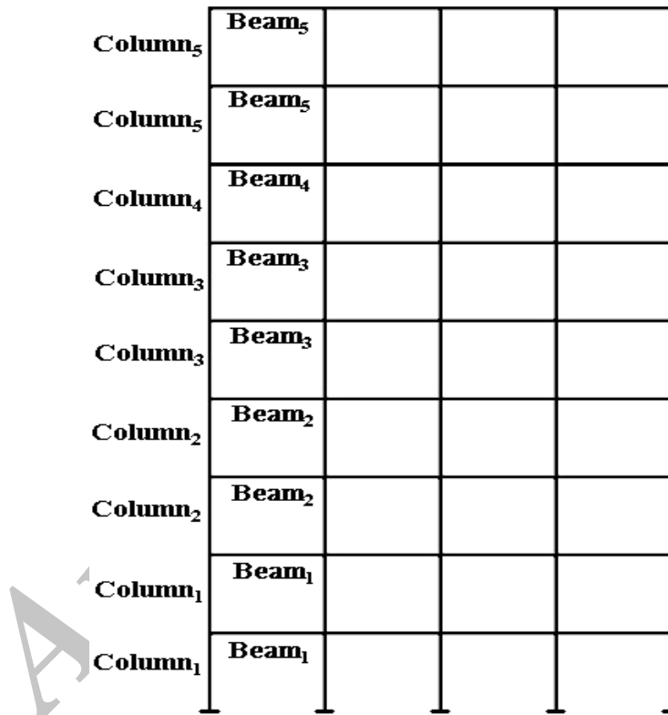
Figure 6. 9-story RC frame
