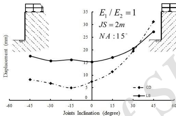
Figure 12. Effect of joints dip on cantilever displacement and lateral bulging, nail angle 15°
