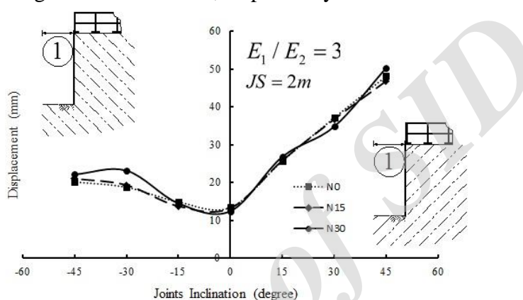
Figure 14. Effect of joints dip on cantilever deflection where anisotropy equals to 3
