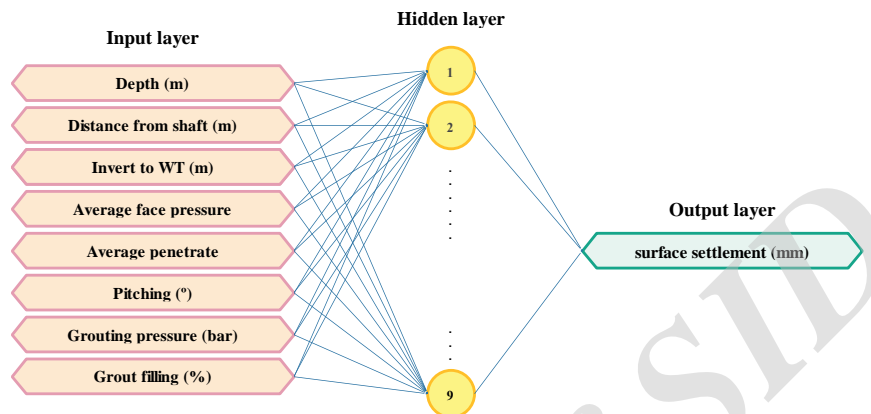
Figure 9. Architecture of ANN-BBO model.
