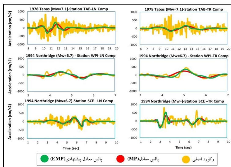
Figure 1. Fitting of acceleration time histories with MP and EMP models
