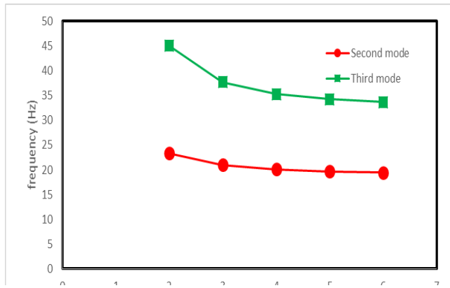
Figure 8. Variation of effective natural frequency versus length to height ratio of the wall
