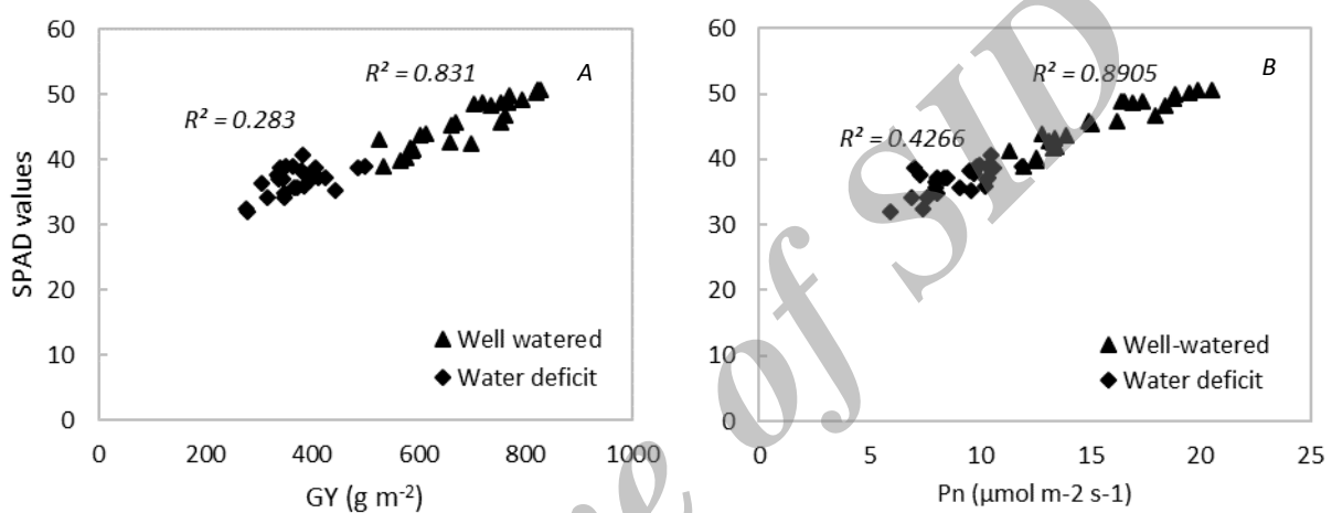
Figure 4. Scattered diagram showing relationship between SPAD values and grain yield (GY) [ \text{g m}^{-2} ] (A) and net photosynthesis rate (Pn) [ \mu\text{mol m}^{-2}\text{s}^{-1} ] (B) of 25 wheat genotypes under well-watered and water deficit conditions. Values represent the means for nine measurements (three measurements in each replication) made on flag leaf
