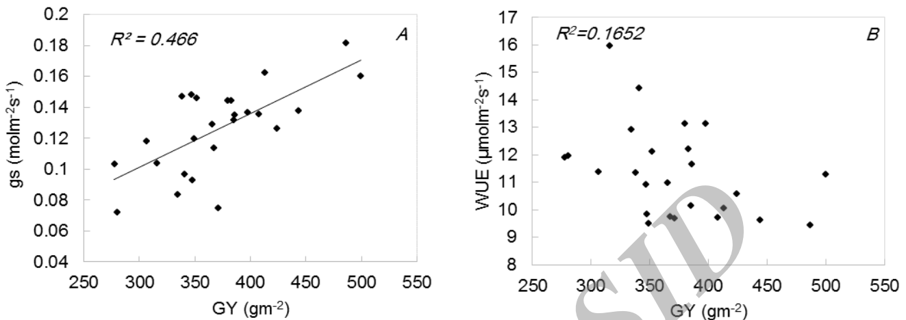
Figure 3. Scattered diagram showing relationship between grain yield (GY) [gm -2 ] and stomatal conductance ( g_s ) [molm -2 s -1 ] (A) and water use efficiency (WUE) [μmolm -2 s -1 ] (B) of 25 wheat genotypes in response to drought stress. Values represent the means for nine measurements (three measurements in each replication) made on flag leaf
