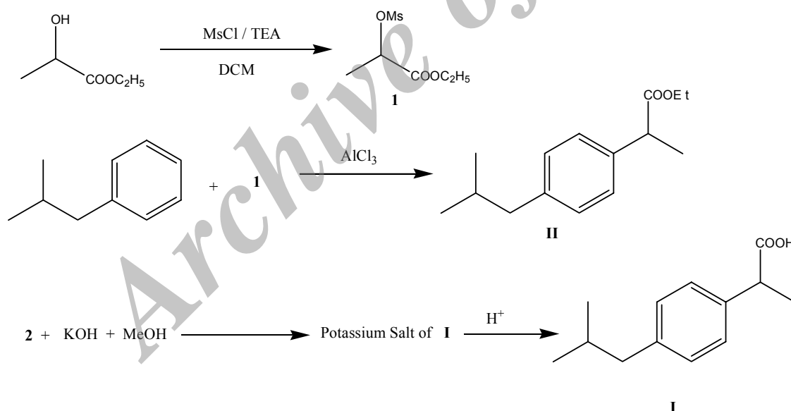
Scheme 2. Our modified method for synthesizing of ibuprofen.
