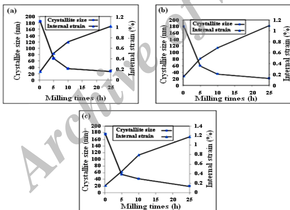
Fig. 3. The crystallite size and the internal strain of WC phase of samples (a) B, (b) C, and (c) D at different milling times
