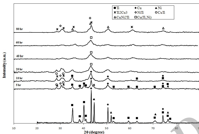
Fig. 1. XRD patterns of the Ti_{50}Cu_{40}Ni_{10} powder alloy after mechanical alloying for 5-80 h
