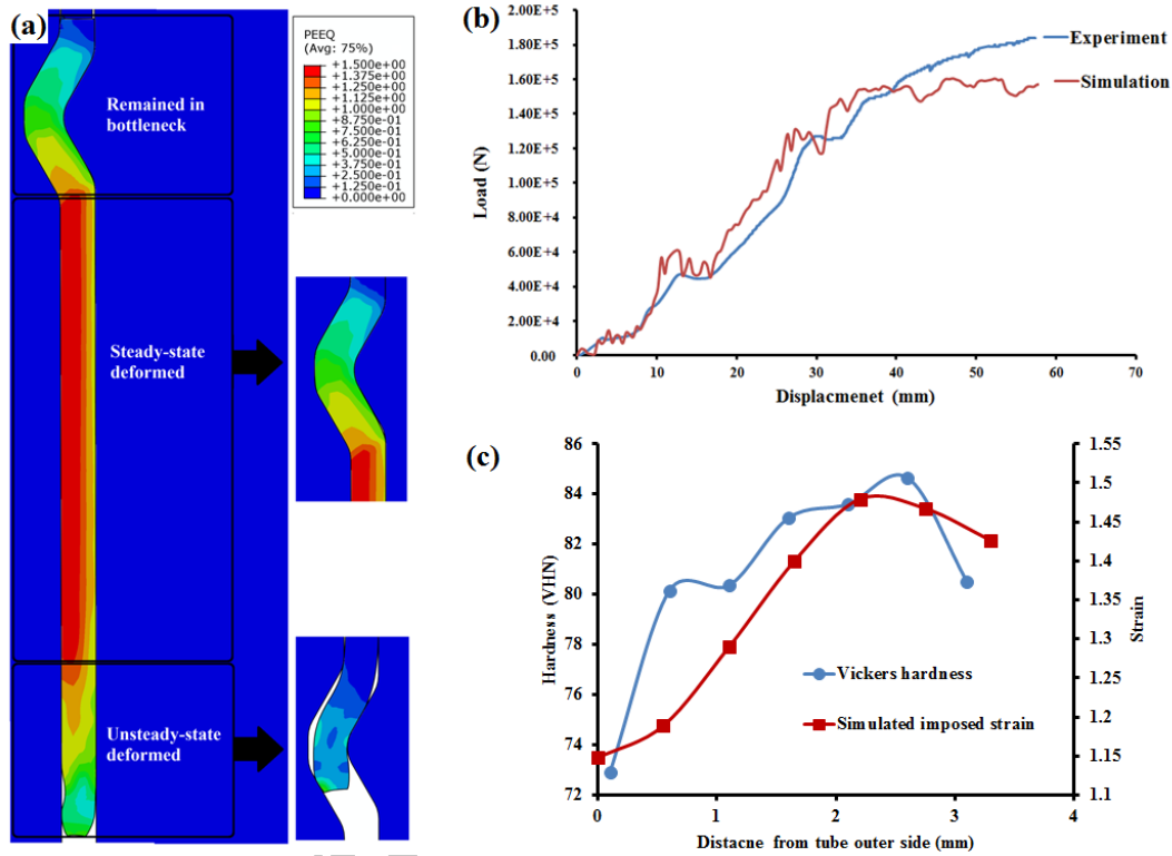
Fig. 3. (a) Illustration of three differently deformed regions through processing by new geometry of TCP. (b) Comparison of simulation and experiment results for load-displacement curve of TCP processing using manufactured die. (c) Comparison of the simulated imposed strain and the Vickers micro-hardness along tube wall thickness after one pass of TCP
