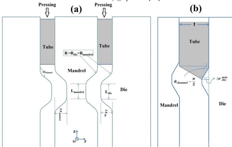
Fig. 1. (a) Schematic illustration of the new geometry of TCP and its geometrical variables. (b) The illustration of minimum of \Delta r_{die} for occurrence of subsequent shear through TCP
