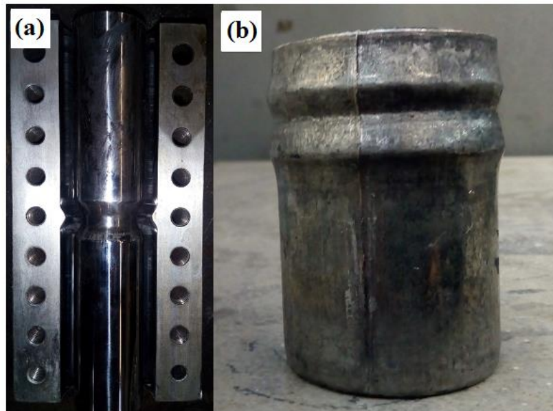
Fig. 2. (a) Manufactured TCP die considering the new geometry. (b) The specimen processed using manufactured die
