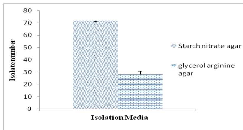
Figure 1: Comparison of isolation of actinobacteria in two isolation media.
