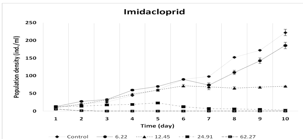
Figure 2: Population density of Brachionus calyciflorus exposed to five concentrations of imidacloprid ( 0.00 (control), 6.22 , 12.45 , 24.91 and 62.27 \text{ mg L}^{-1} ) at 10 days. The values are mean±standard error and shown based on three replicate recordings.
