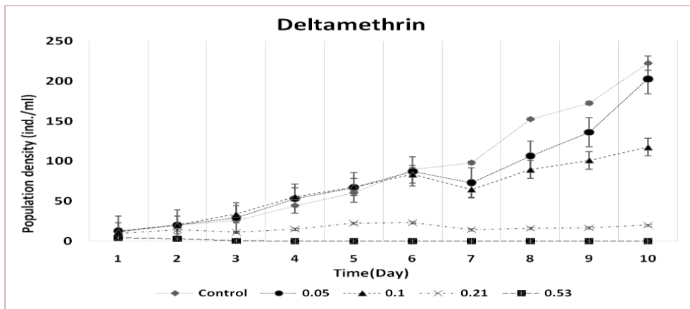
Figure 1: Population density of Brachionus calyciflorus exposed to five concentrations of deltamethrin ( 0.00 (control), 0.05 , 0.1 , 0.21 and 0.53 \text{ mg L}^{-1} ) at 10 days. The values are mean±standard error and shown based on three replicate recordings.
