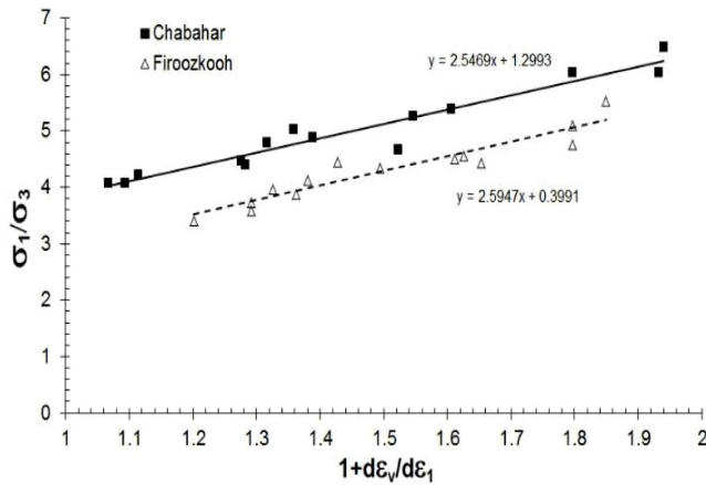
Fig. 6. Maximum and minimum principal stress ratio versus dilation parameters
