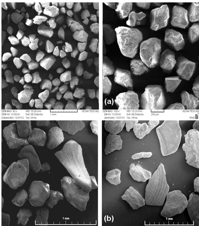
Fig. 2. Microscopic electronic images of sands: (a) Firoozkoh (b) Chabahar sand
