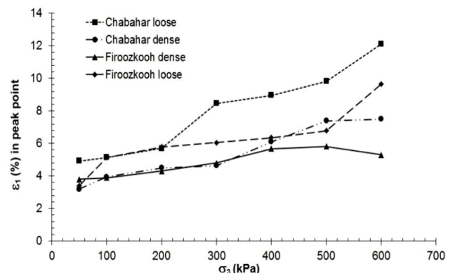
Fig. 4. Axial strain at peak point versus confining stress
