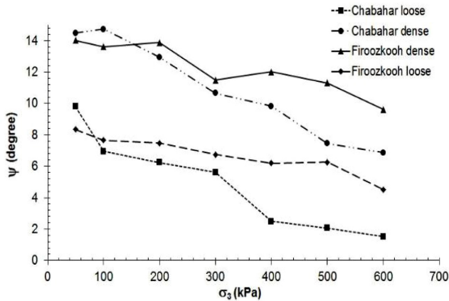
Fig. 5: Dilation angle versus confining pressure
