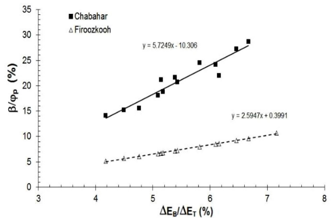
Fig. 8. Particle breakage angle to peak internal friction angle versus consumed energy for particle breakage to total applied energy
