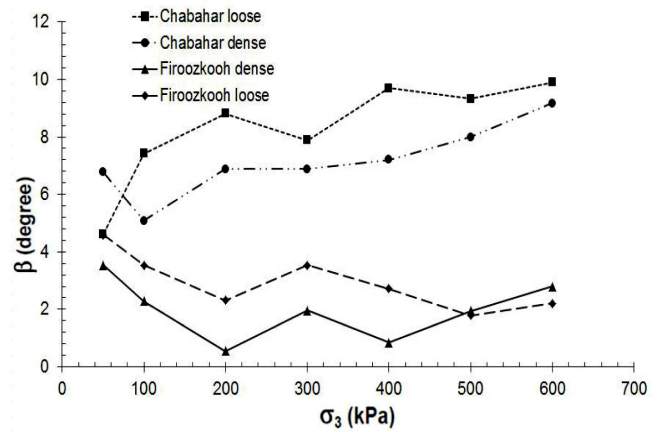
Fig. 7. Particle breakage angle versus confining pressure
