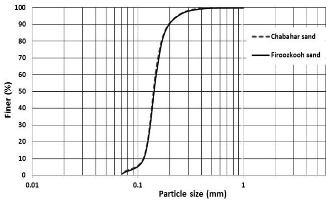
Fig. 1. Particle size distribution of sands
