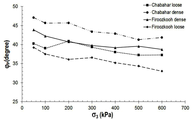
Fig. 3. Internal friction angle versus confining pressure
