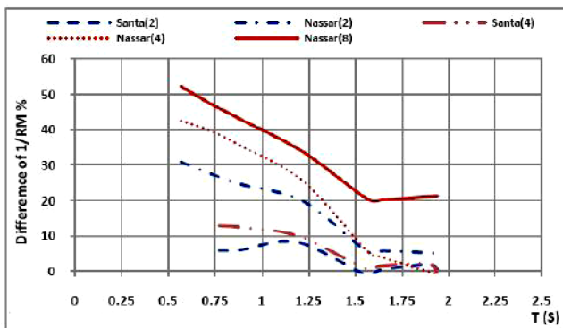
Fig. 2. Comparison of ductility modification factor ( 1/R_M ) for near fault ground motion proposed in this study with those in previous investigation for far fault ground motions [2,6].
