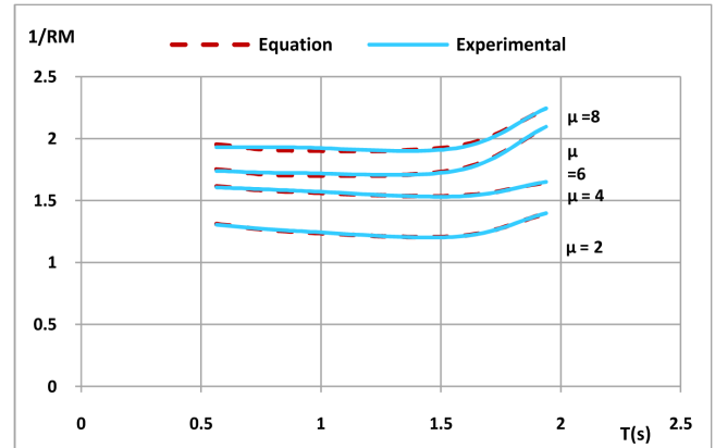
Fig. 3. Comparisons of fitting curves of this study with the previous investigations [2, 6].
