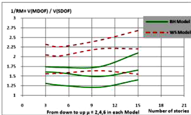
Fig. 1. Influence of failure mechanism on ductility modification factor
