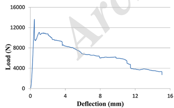
Figure 3: Load-deflection diagram for lightweight concrete with 0.4% of industrial steel fibres and 0.1% of glass fibres
