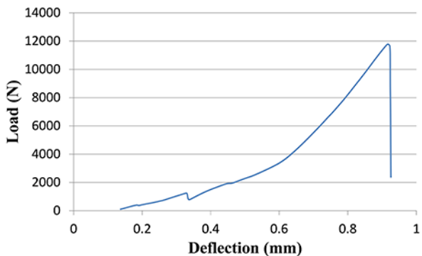
Figure 1: Load-deflection diagram for conventional (control) concrete
