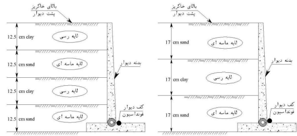
Figure 2. Details of soil layering behind the wall
