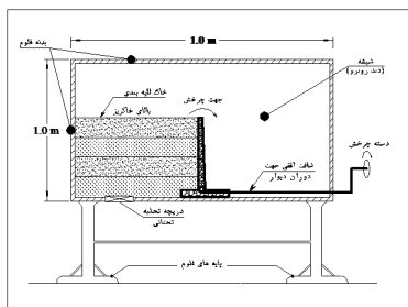
Figure 1. Cross section of the laboratory model
