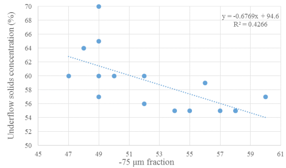
Figure 6. The effect of -75 μm fraction of a deep bed thickener discharge solids concentration
