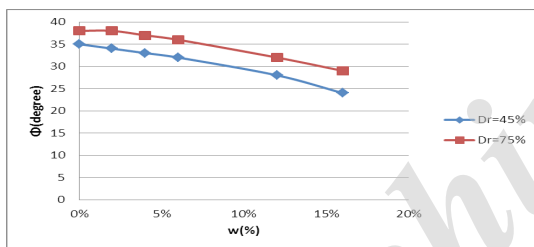
Figure 1. The changes of the internal friction angles in different gasoil content
