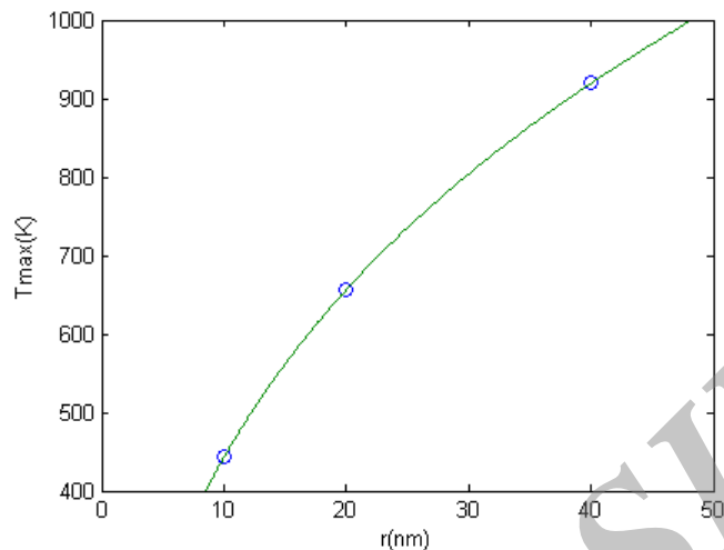
Figure 2: Interpolation of maximum temperature for the range of particle size from 10 nm to 40 nm
