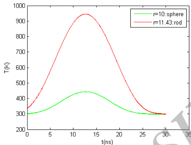
Figure 4: Temperature versus time for a nanorod (reff=11.43 nm) and a nanosphere (r=10 nm)
