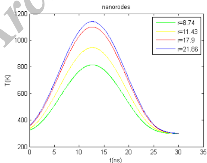
Figure 3: Temperature profile versus time for nanorods with different effective radius
