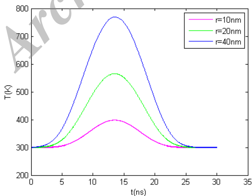
Figure 1: Particle temperature versus time for particles with 10, 20 and 40 nm radius
