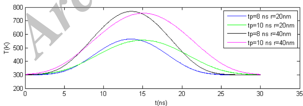
Figure 5: Temperature versus time for nanoparticles with radiuses of 20 and 40 nm at the width pulses of 8 and 10 ns
