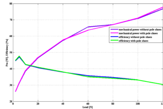
Fig. 8. b. Variation of Pm, efficiency with load
