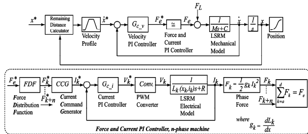
Fig. 6. Control block diagram for the proposed LSRM
