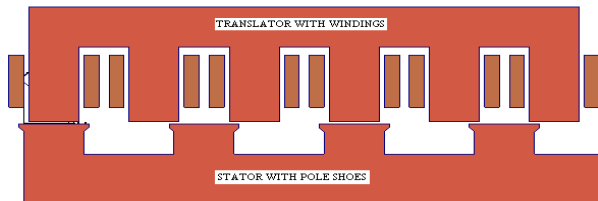
Fig. 4. 2D Cross sectional view of the proposed LSRM
