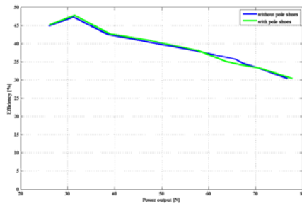
(c) Fig. 8. c. Variation of efficiency with P_m
