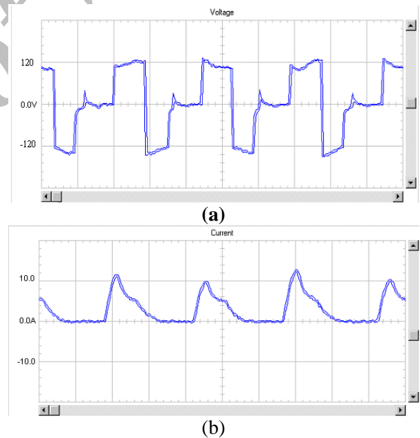
Fig. 11. Experimental waveforms during single pulse operation (a) Actual phase voltage of LSRM (b) Actual phase current of LSRM
