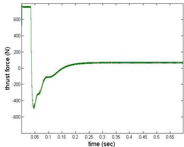
Fig.12. Reference and real forces in proposed DTC method.
