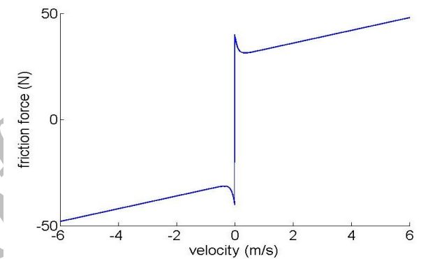
Fig.7. Relation of friction and velocity by using the simulation of a mathematical relation.
