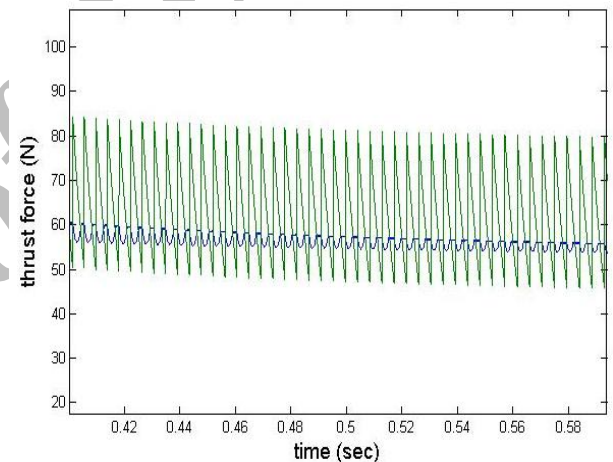
Fig.11. Reference and real forces in DTC method by magnification
