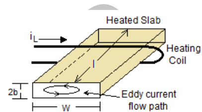
Fig. 2. Model of slab for one turn coil.
