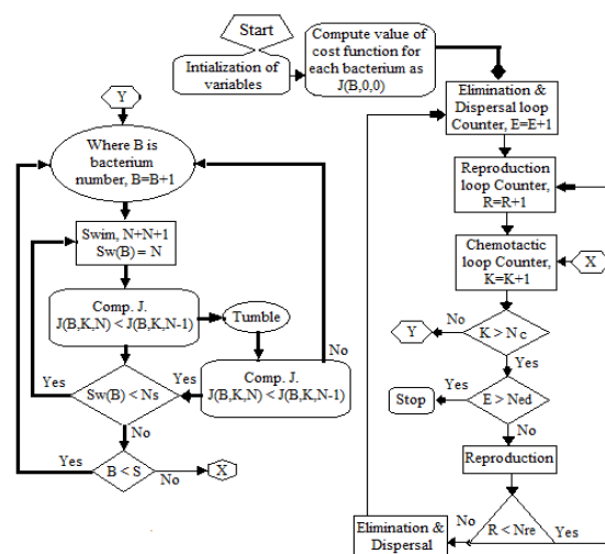
Fig.4. The flowchart of SBFA.
