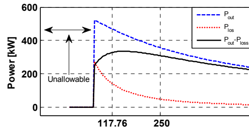
Fig. 6. courses of output power, power loss and difference between both of them.
