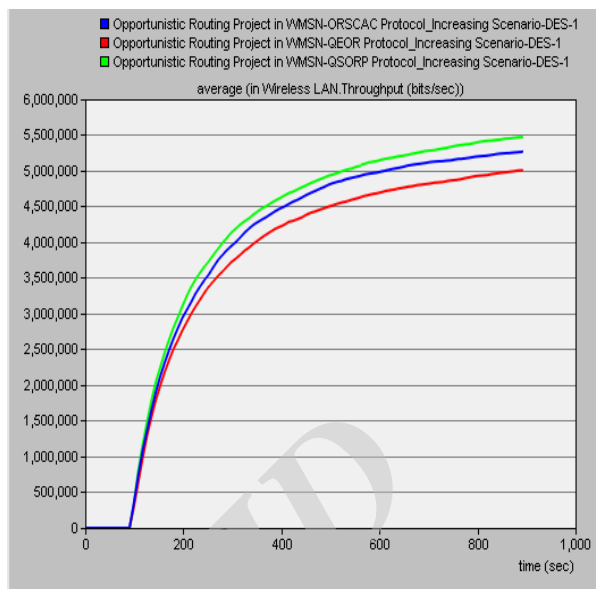
Fig. 6. c. The rate of received data in the compared protocols in increasing scenarios.
