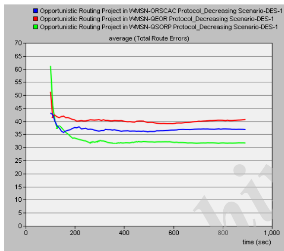
Fig. 3. a. The instability rate of routes in the compared protocols in decreasing scenarios.
