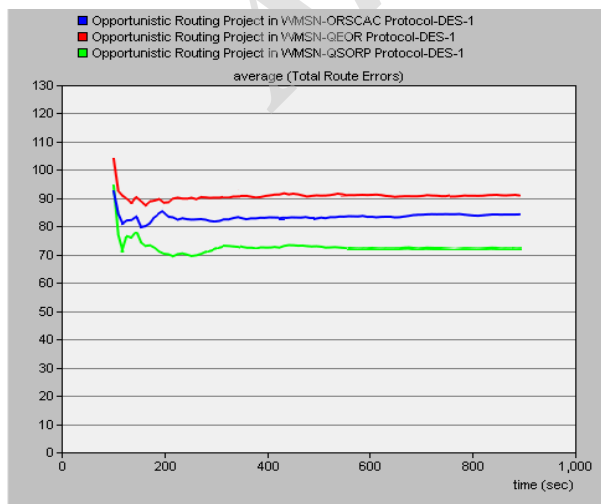
Fig. 3. a. The instability rate of routes in the compared protocols in decreasing scenarios.
