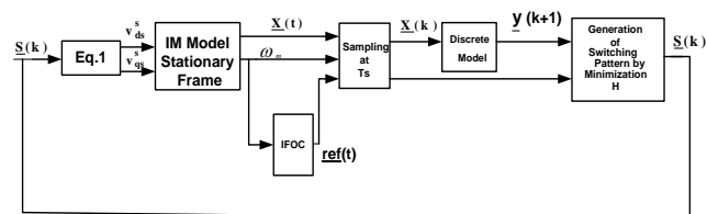
Fig.5 The block diagram of Optimal Controller.
