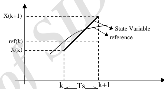
Fig.3. Principle of tracking problem by optimal controller.
