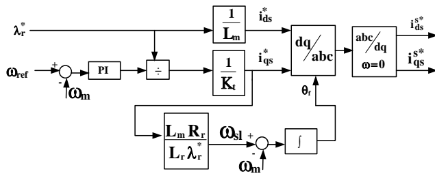
Fig. 1. The block diagram of IFOC.
