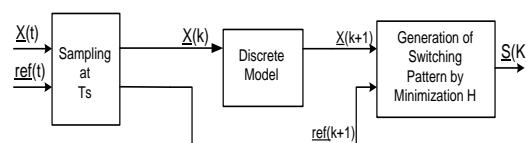
Fig. 4. The Block diagram of switching pattern generation method.
