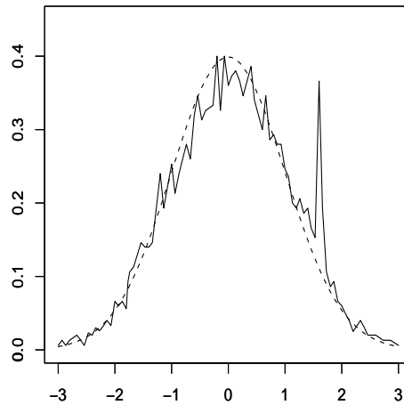
Figure 1: L.T.D.E. for Gaussian process (simulation, [25])
