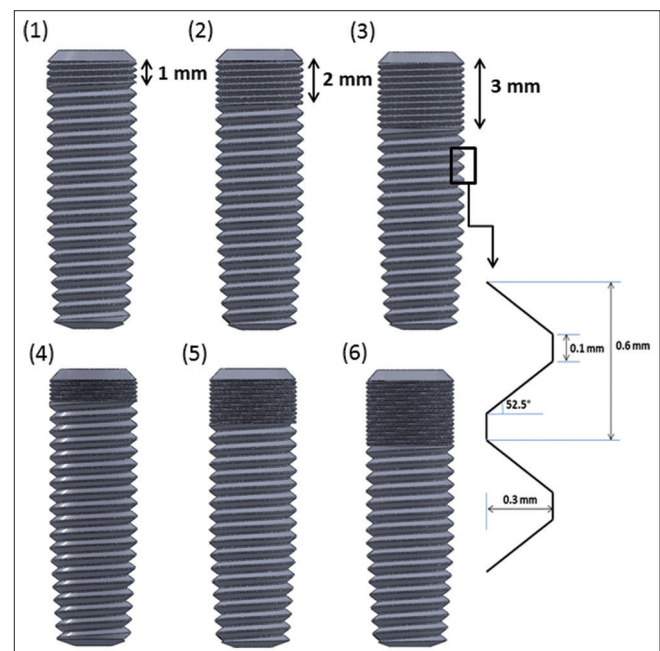
Figure 1: The solid models of six implant models and the design properties of main threads.
