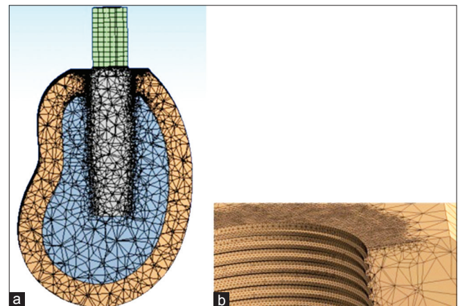
Figure 2: Cross-sectional view of the meshed model (a) and close-up view of the mesh in cortical bone adjacent to implant surface (b).
