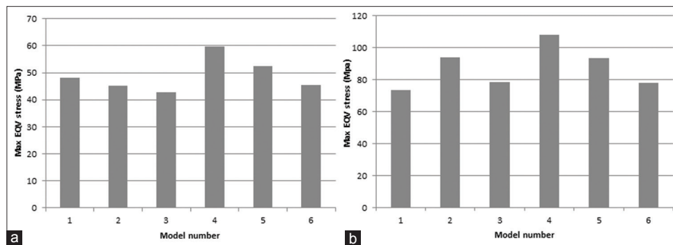
Figure 3: Maximum equivalent stress in cortical bone under axial (a) and oblique (b) loads.
