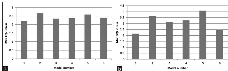
Figure 4: Maximum equivalent stress in cancellous bone under axial (a) and oblique (b) loads.
