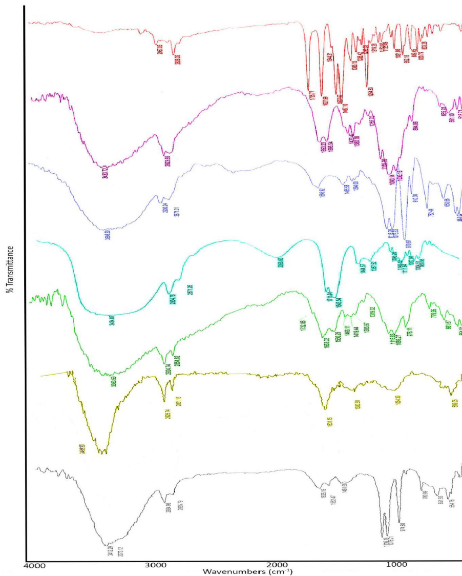
Figure 3. The FTIR spectra of A: ENR, B: Chitosan, C: β-GP, D: Glutaraldehyde E: Chitosan/β-GP, F: Chitosan/Glutaraldehyde, G: single-layer formulation.
