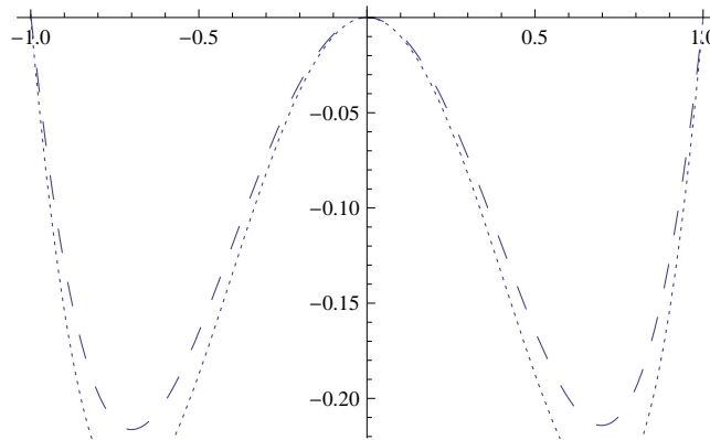
Fig.2. Numerical solution ( \dots ) V_{10}(x) and exact solution ( --- ) v(x) of example 1.
