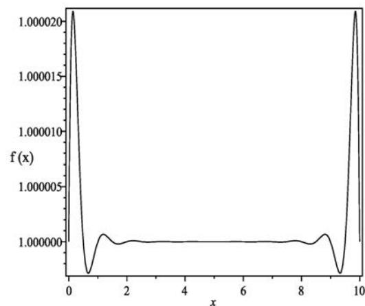
Figure 8: Graph of approximated of f(x) = 1 by using GA-RBF with N = 20 and \epsilon = 0.5 on uniform grid
