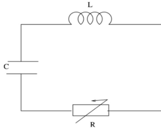
Figure 1: Electric circuit modeling the Van der Pol oscillator in an autonomous regime.
